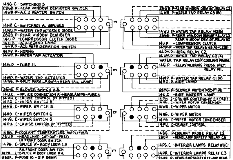
RIGHT-HAND VALANCE LOOM
