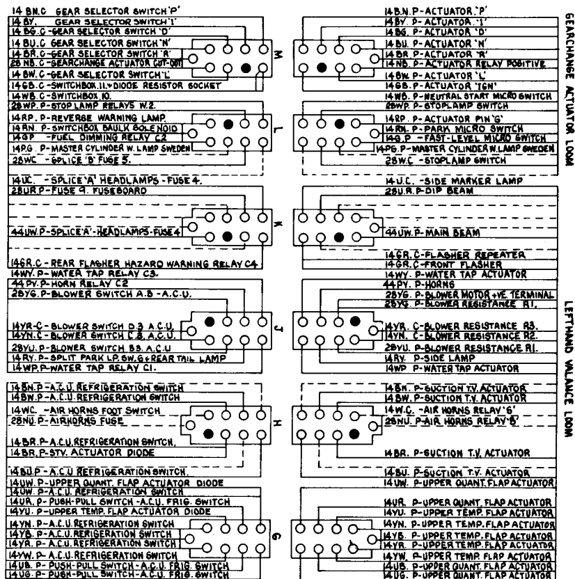
MAIN DISTRIBUTION LOOM LEFT-HAND TOEBOARD SOCKET CONNECTIONS
