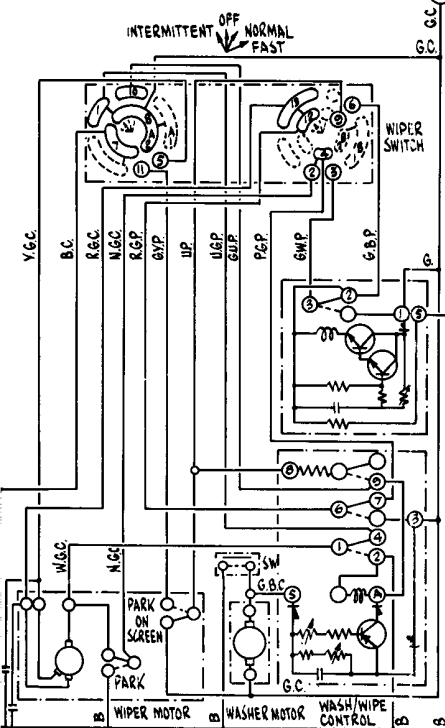
WINDSCREEN WIPER (INCLUDING INTERMITTENT OPERATION) AND WASHER
